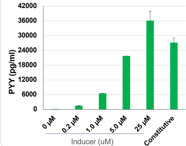
PYY expression
