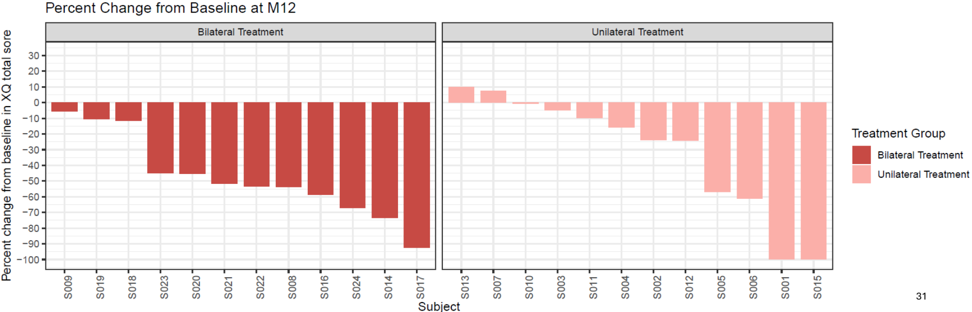
Percent Change from Baseline
