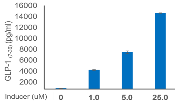
GLP-1 activity specifically on GLP-1 receptor
