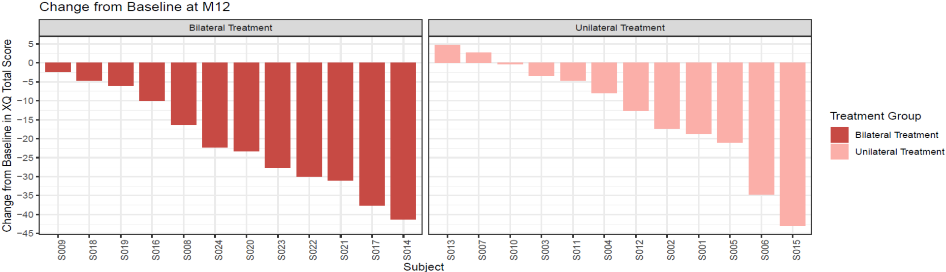
Absolute Change from Baseline
