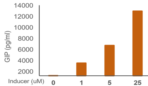
GIP activity specifically on GIP receptor
