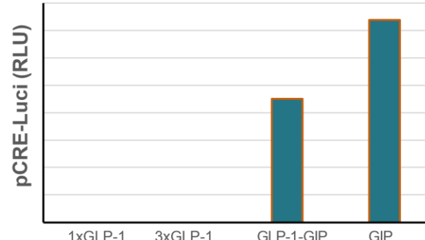
GIP activity specifically on GIP receptor
