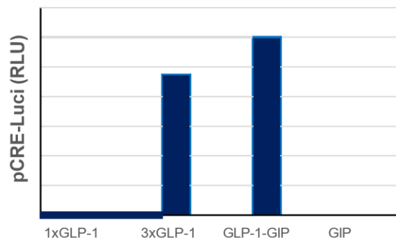
GLP-1 activity specifically on GLP-1 receptor
